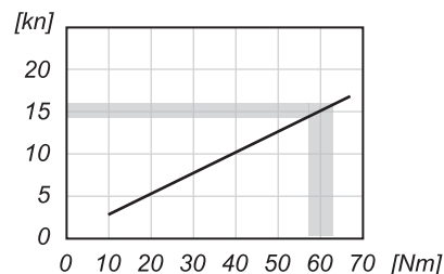
( CLAMPING CURVE )
